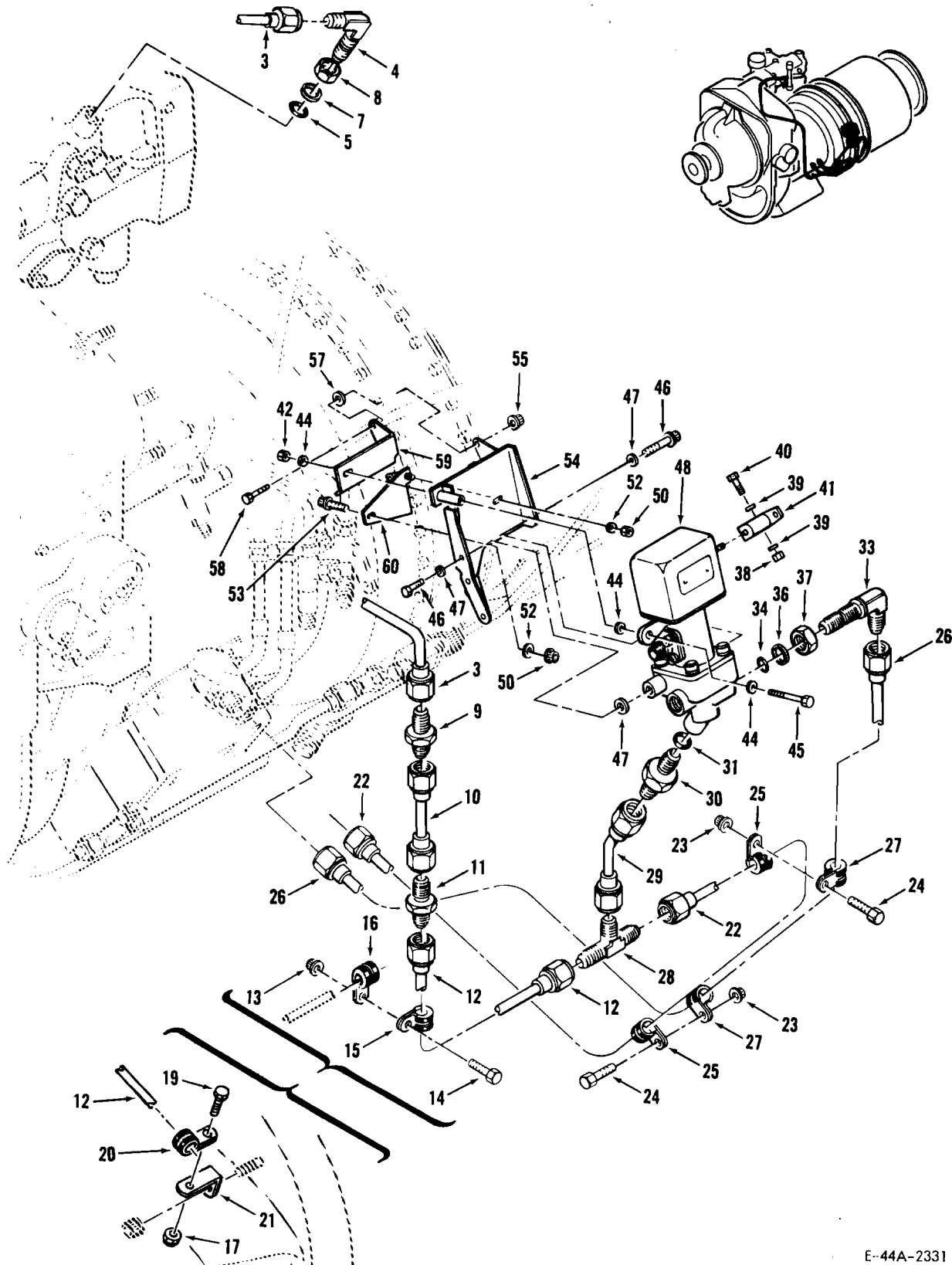
(Code CA-CV) Fuel Shutoff Valve and Plumbing Figure 3
