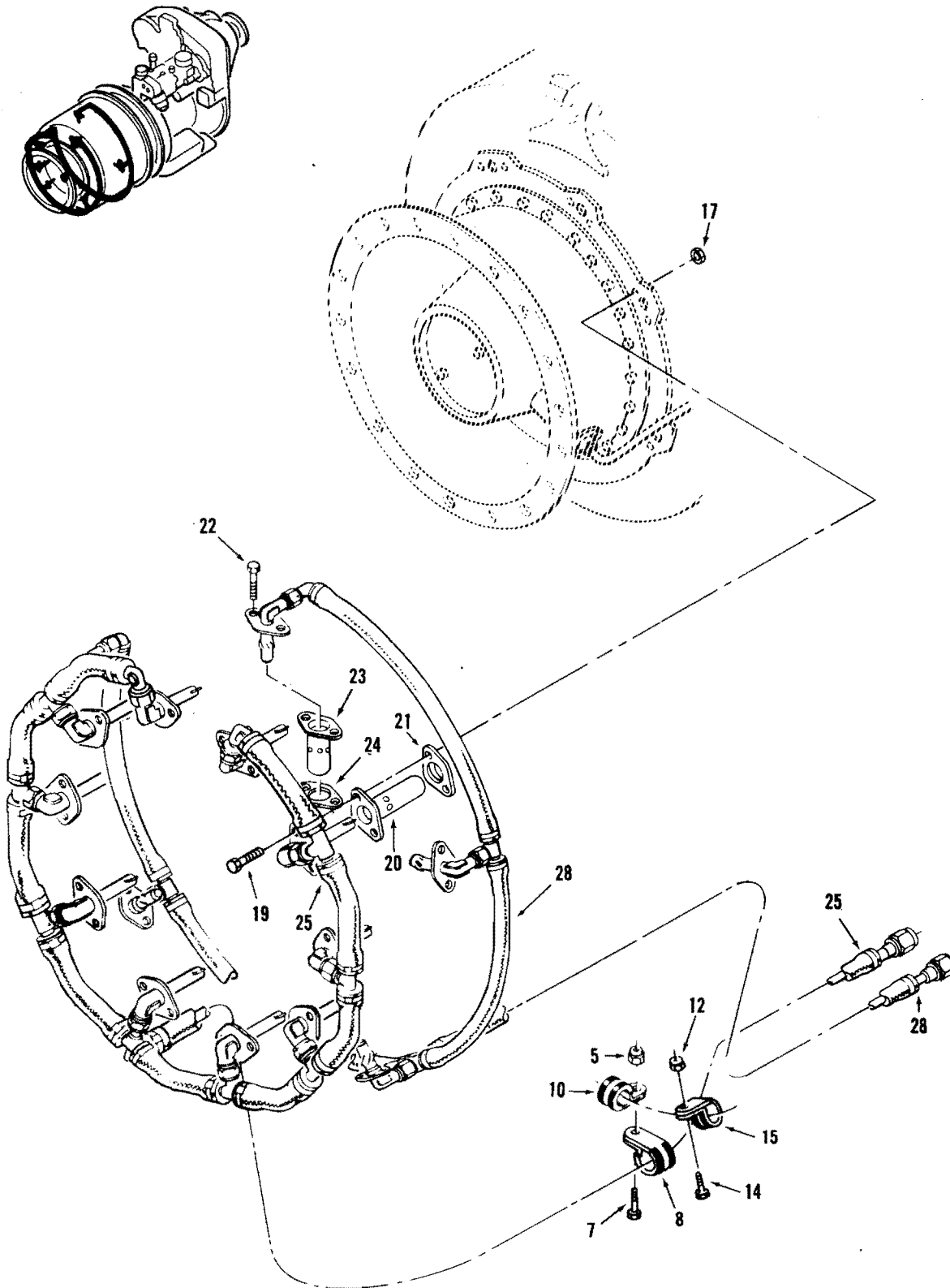
Fuel Nozzle and Manifold Assemblies Figure 1
