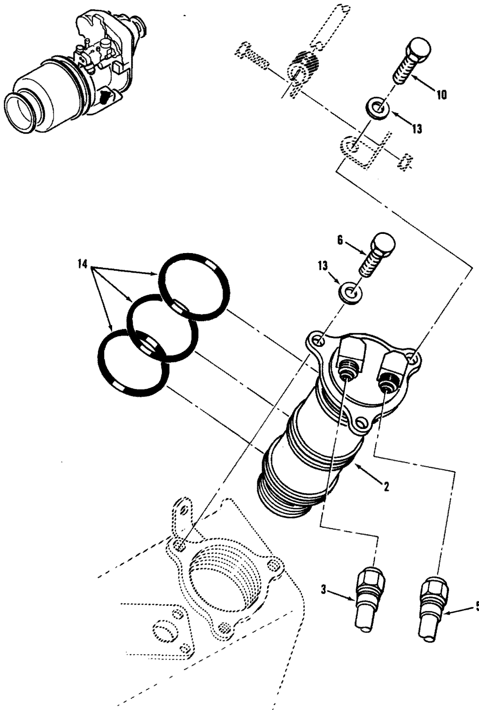
Oil to Fuel Cooler Figure 2
