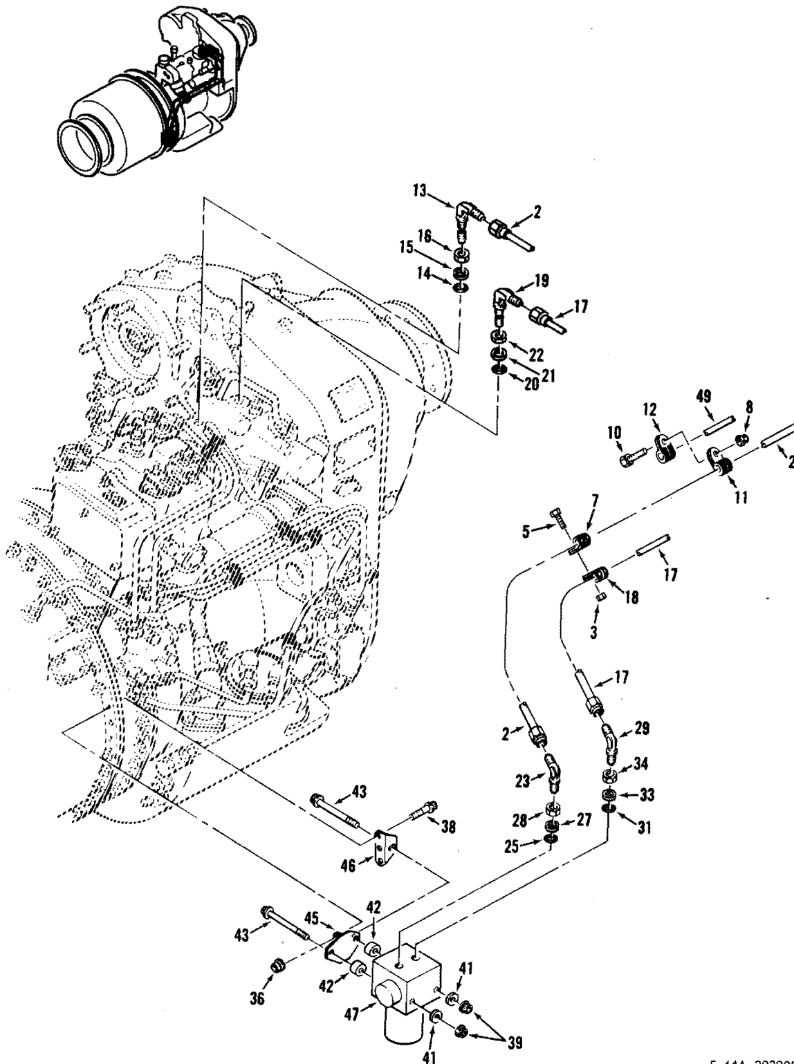
(Code AA-AV) Fuel Filter Installation Kit Figure 1
