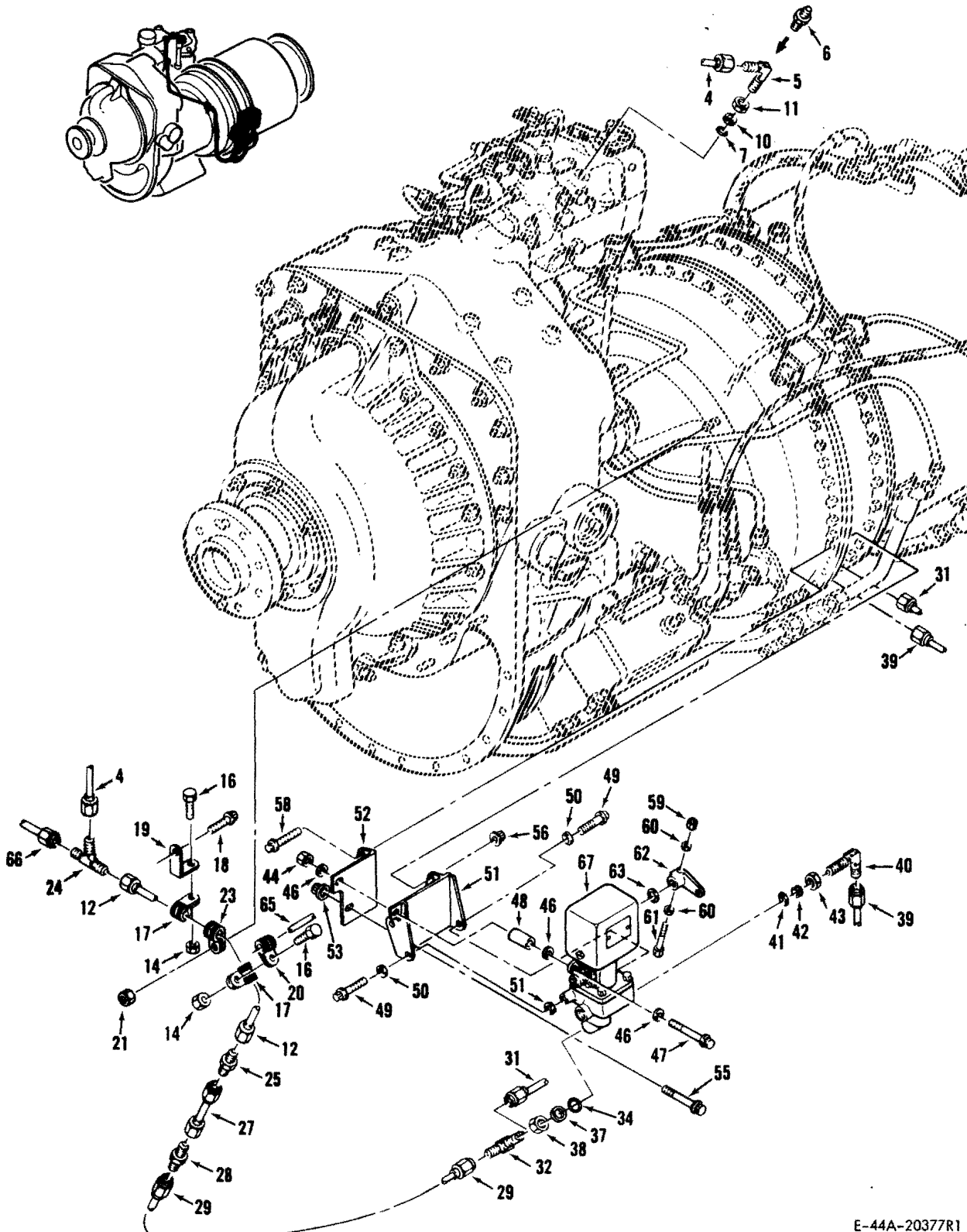
(Code AA-AV) Fuel Shutoff Valve and Plumbing Figure 1
