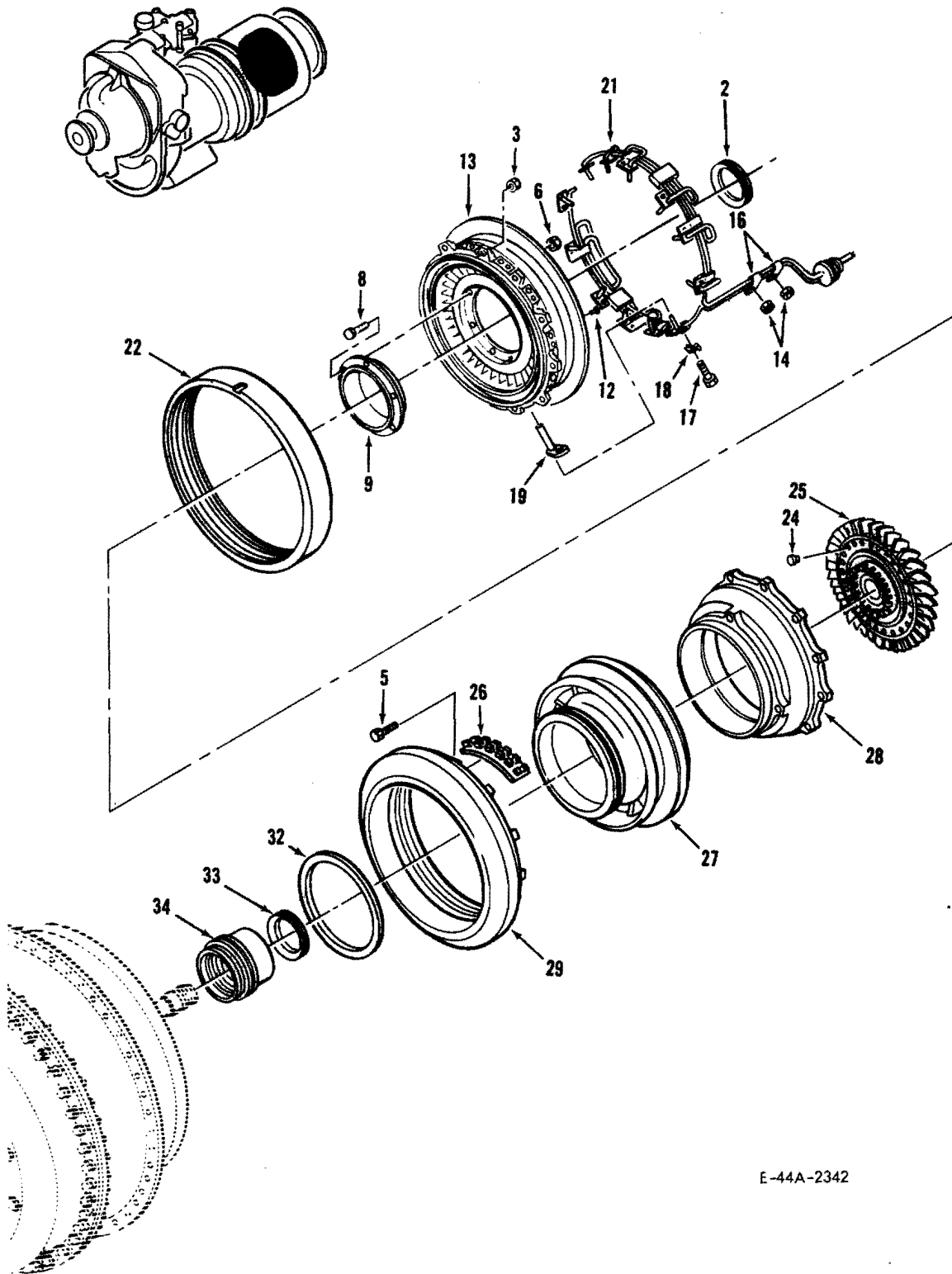
First Stage Turbine Wheel and First and Second Stage Stator Assemblies Figure 10
