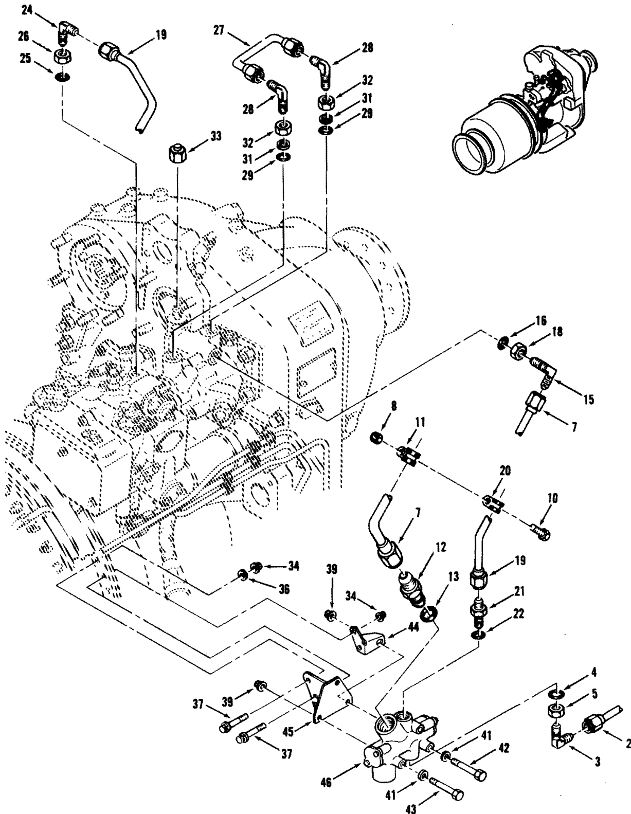
(Code CA-CV) Anti-Icing Valve and Plumbing Figure 2
