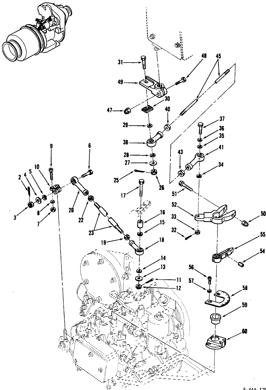
Control Linkage Assembly Figure 1
