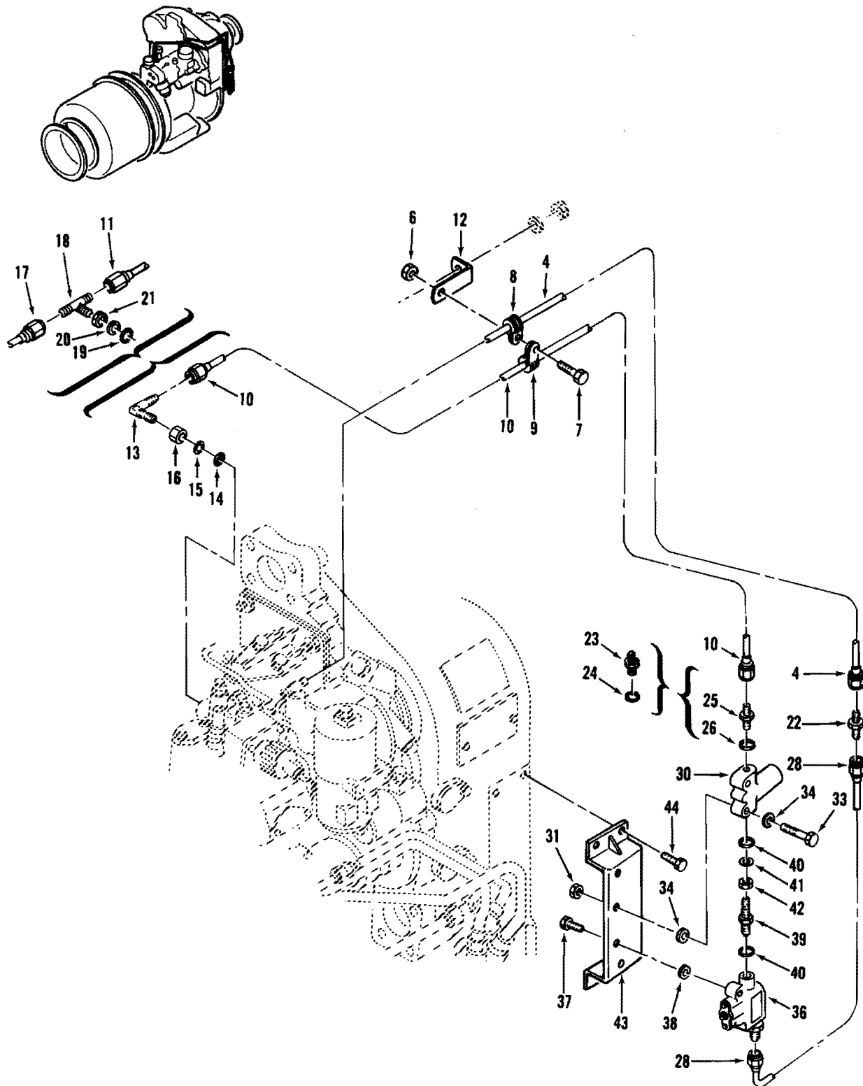
(Code BA-BV) Fuel Pressure Regulator and Plumbing Figure 1
