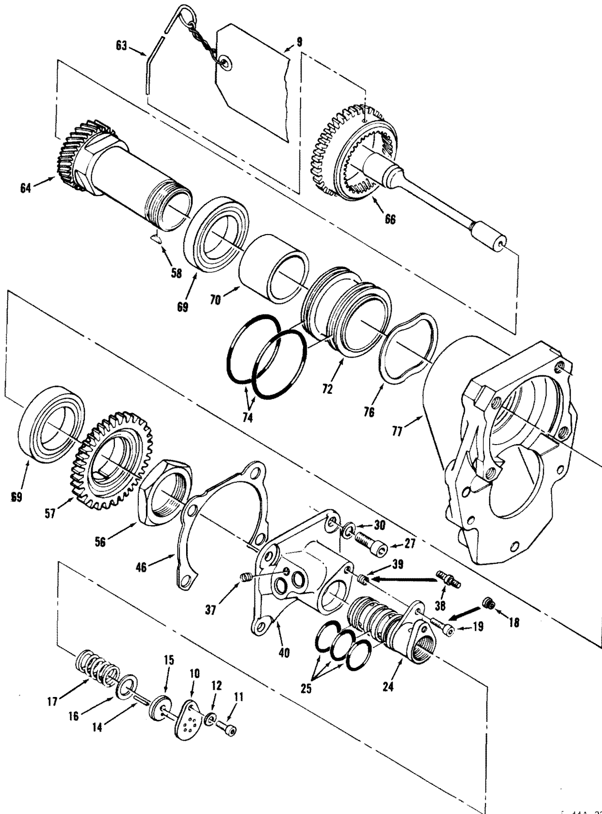
Torque Sensor Assembly Figure 1
