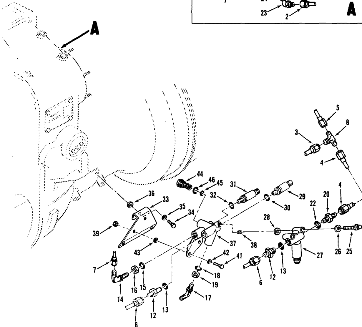
(Code CA-CV) Pressure Switch and Negative Torque Sensor Housing Installation Kit Figure 3
