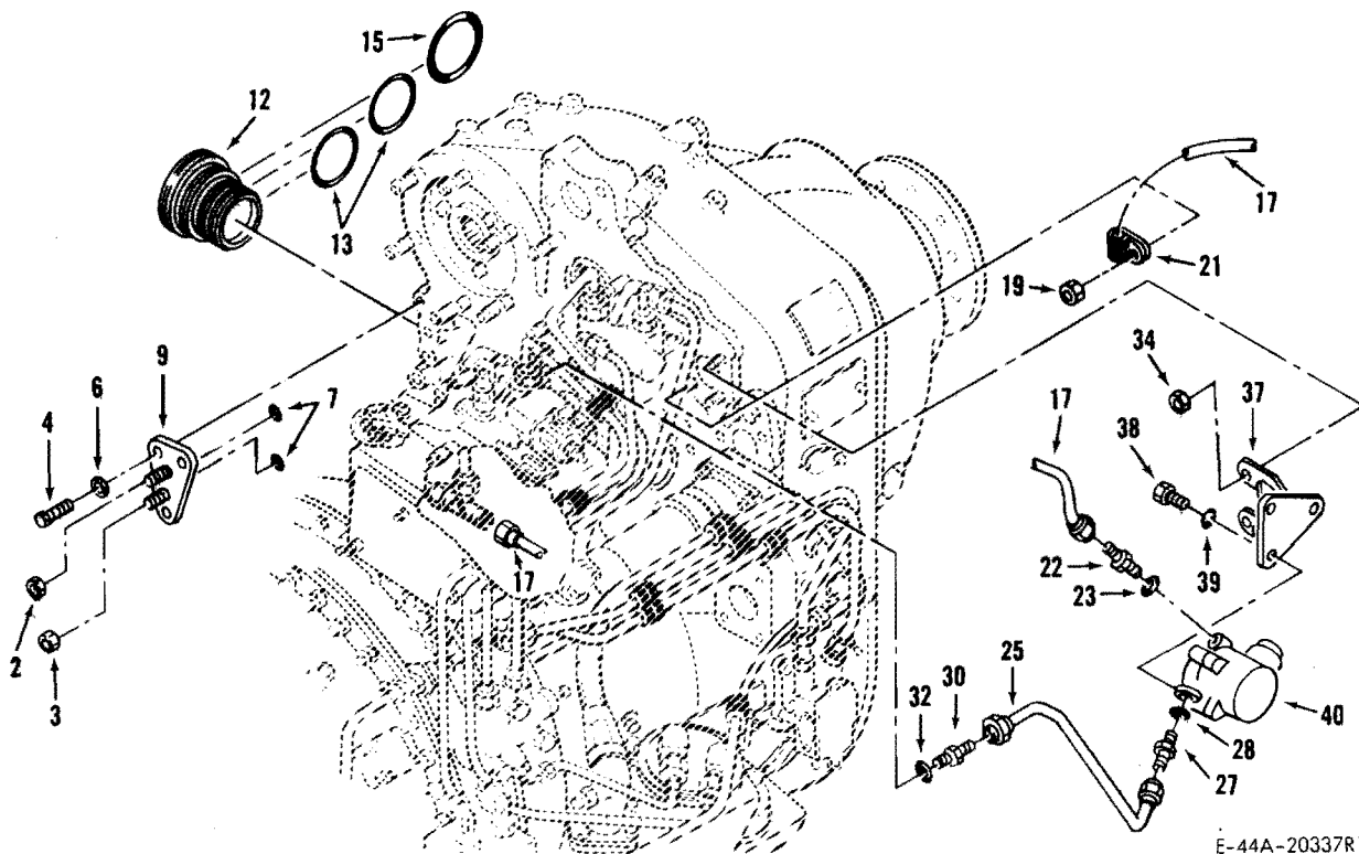
(Code AA-AV) Torque Limiter Installation Kit Figure 1
