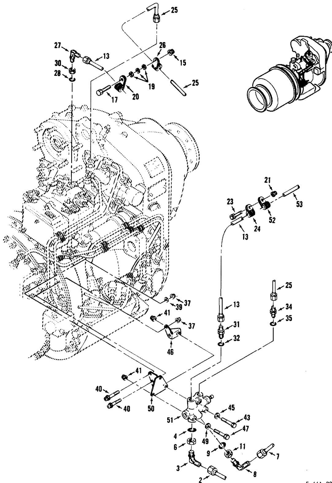
(Code AA-AV) Anti-Icing Valve and Plumbing Figure 1
