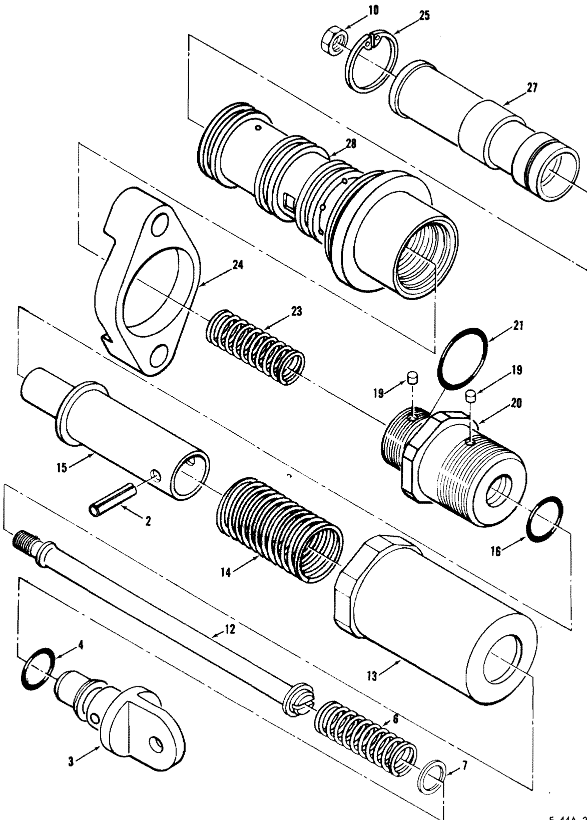
Feathering Valve Figure 1
