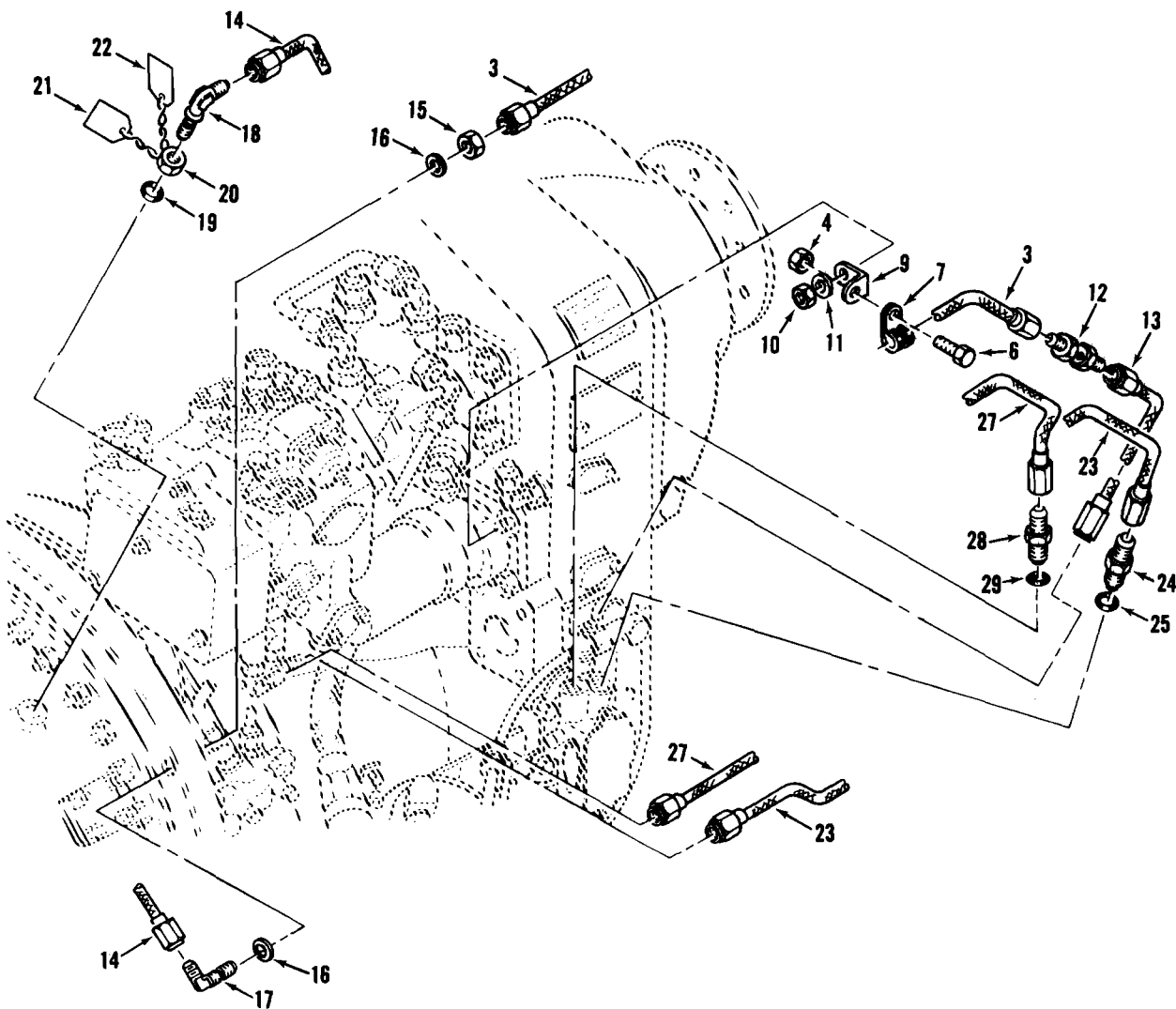
(Code CA-CV) Fuel System Lines Figure 3
