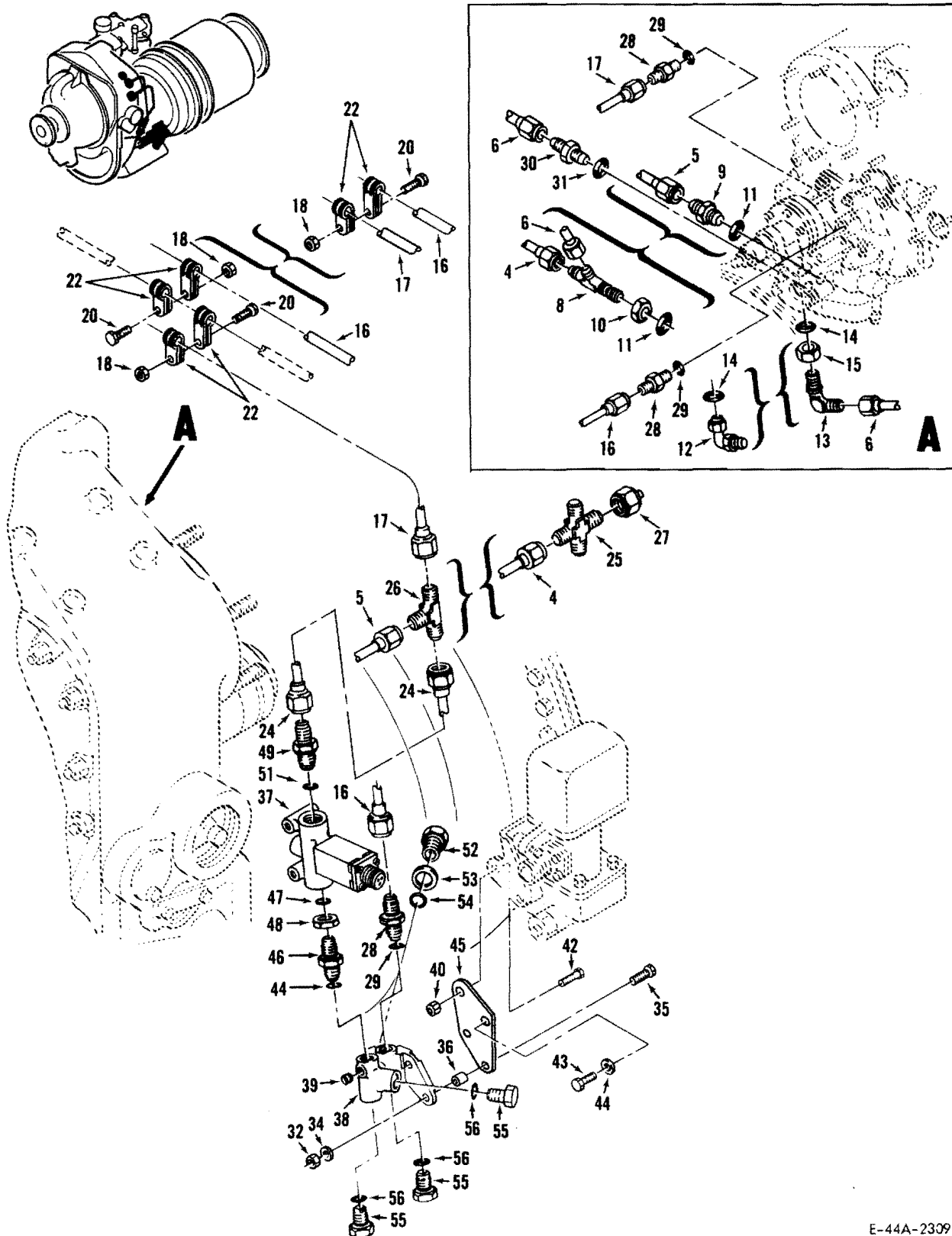
(Code AA-AV) Pressure Switch Housing Installation Figure 1
