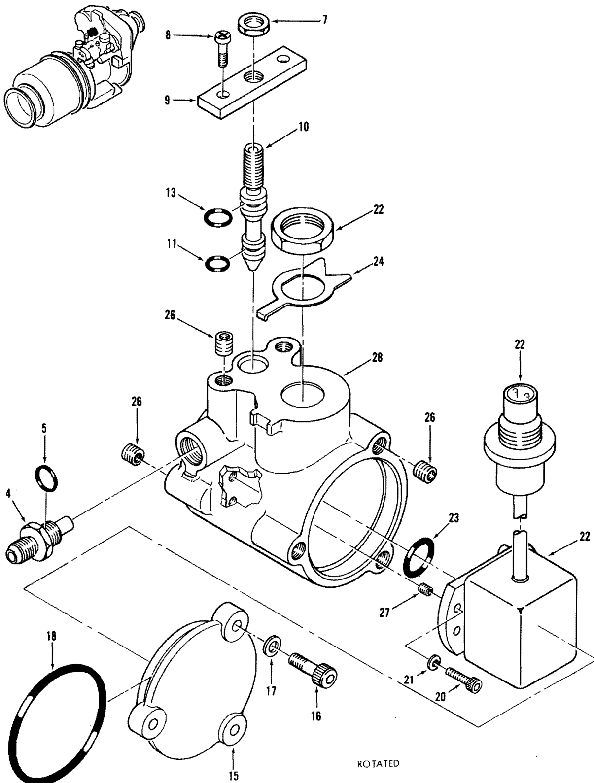
(Codes AA-AV, BA-BV) Torque Limiter Assembly Figure 4
