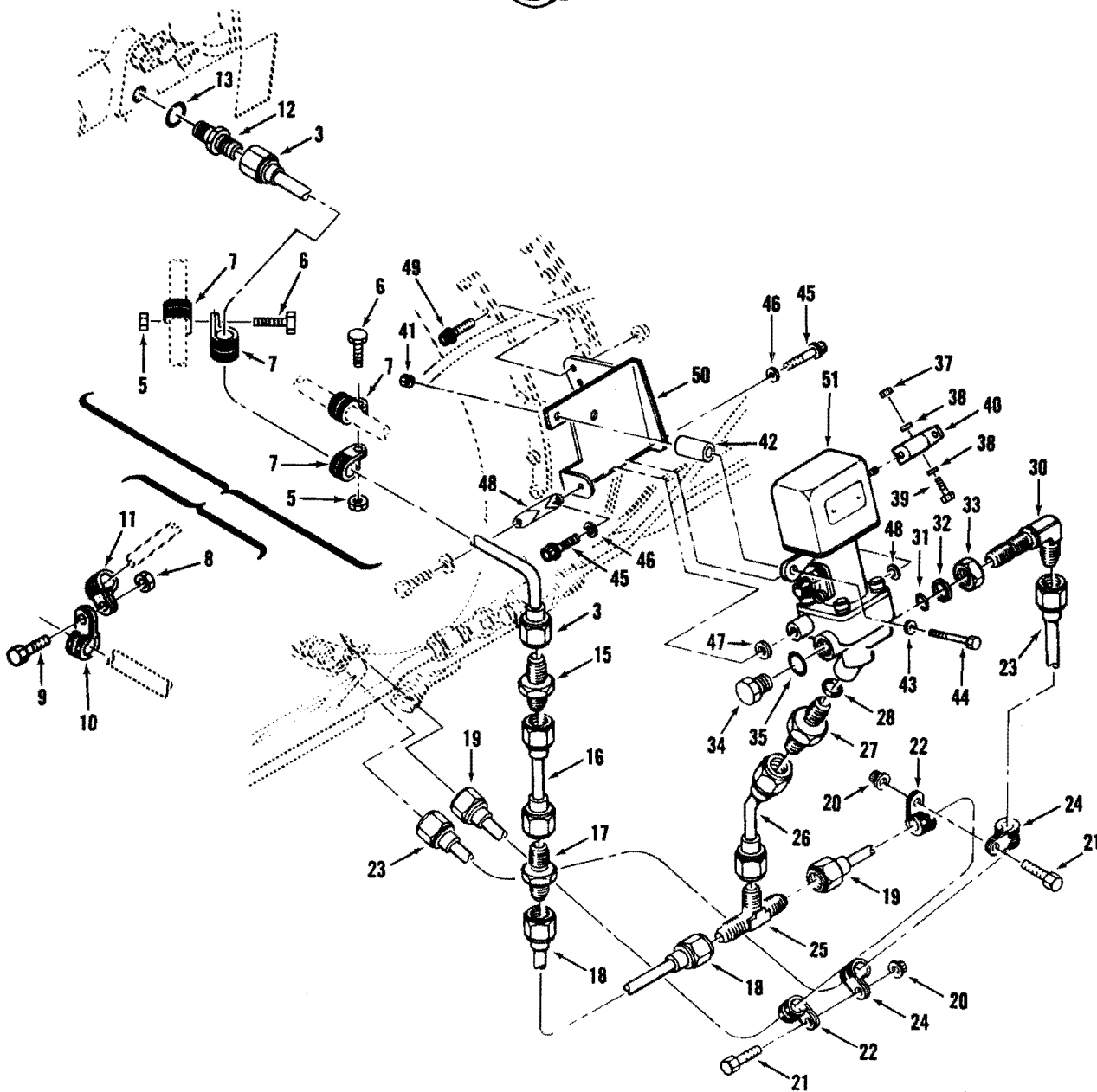
Code BA-BV) Fuel Shutoff Valve and Plumbing Figure 2
