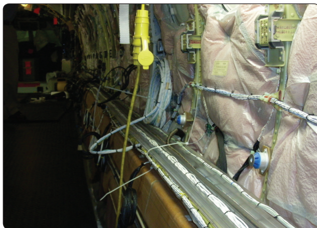
Figure 9-147. Wire lacing.
