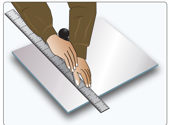
Figure 4-16. Awl usage.
