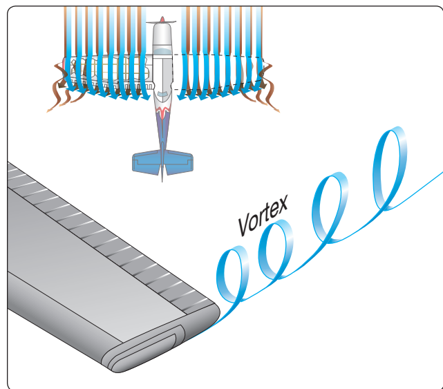
Figure 2-9. Wingtip vortices.
