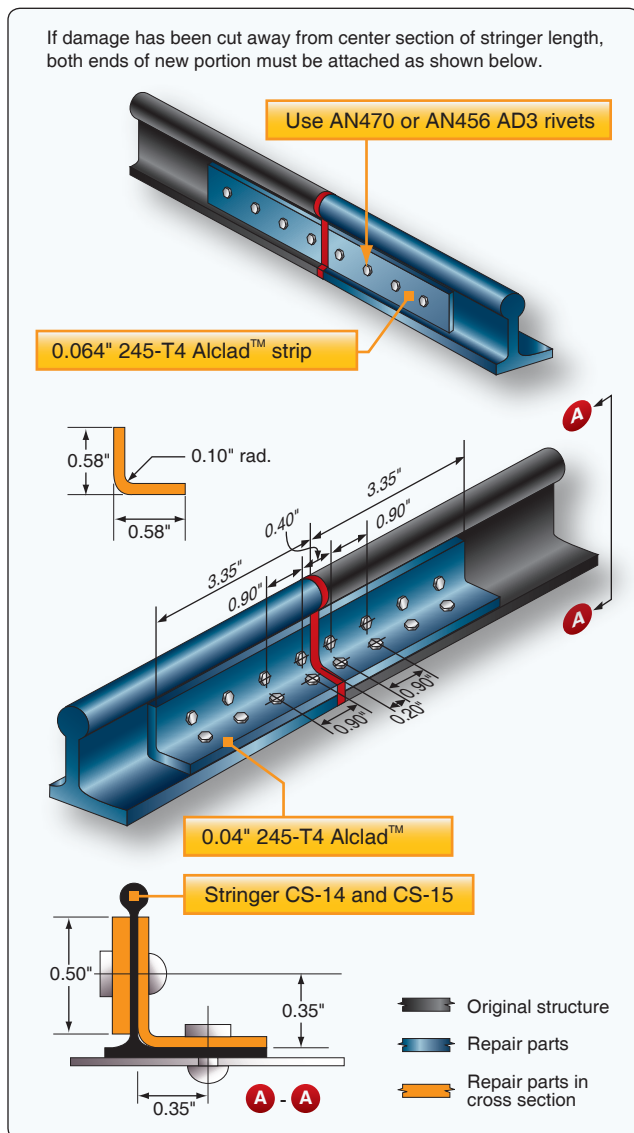
Figure 4-183. Stringer repair.
