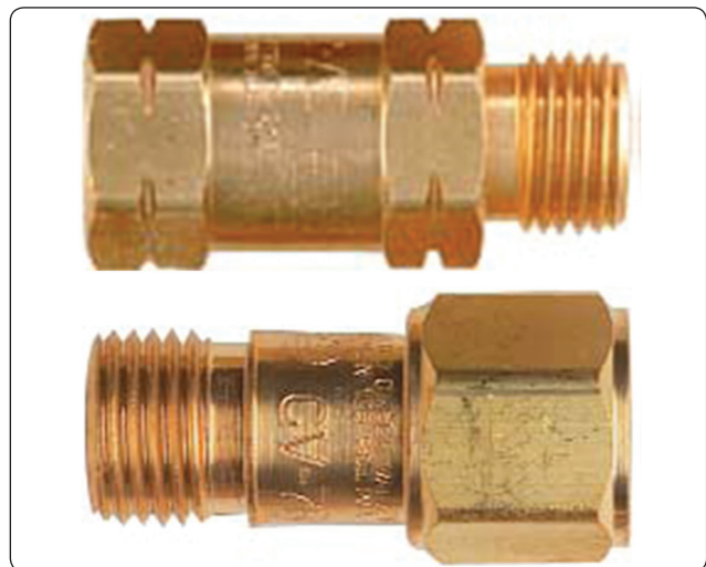
Figure 5-15. Check valves.
