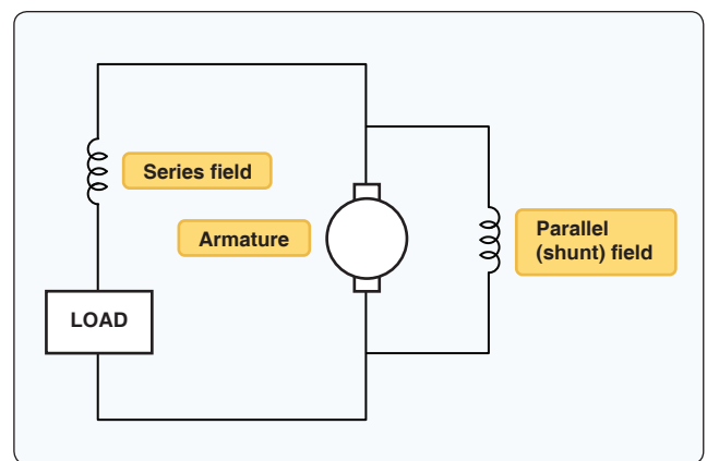
Figure 9-55. Starter-generator.
