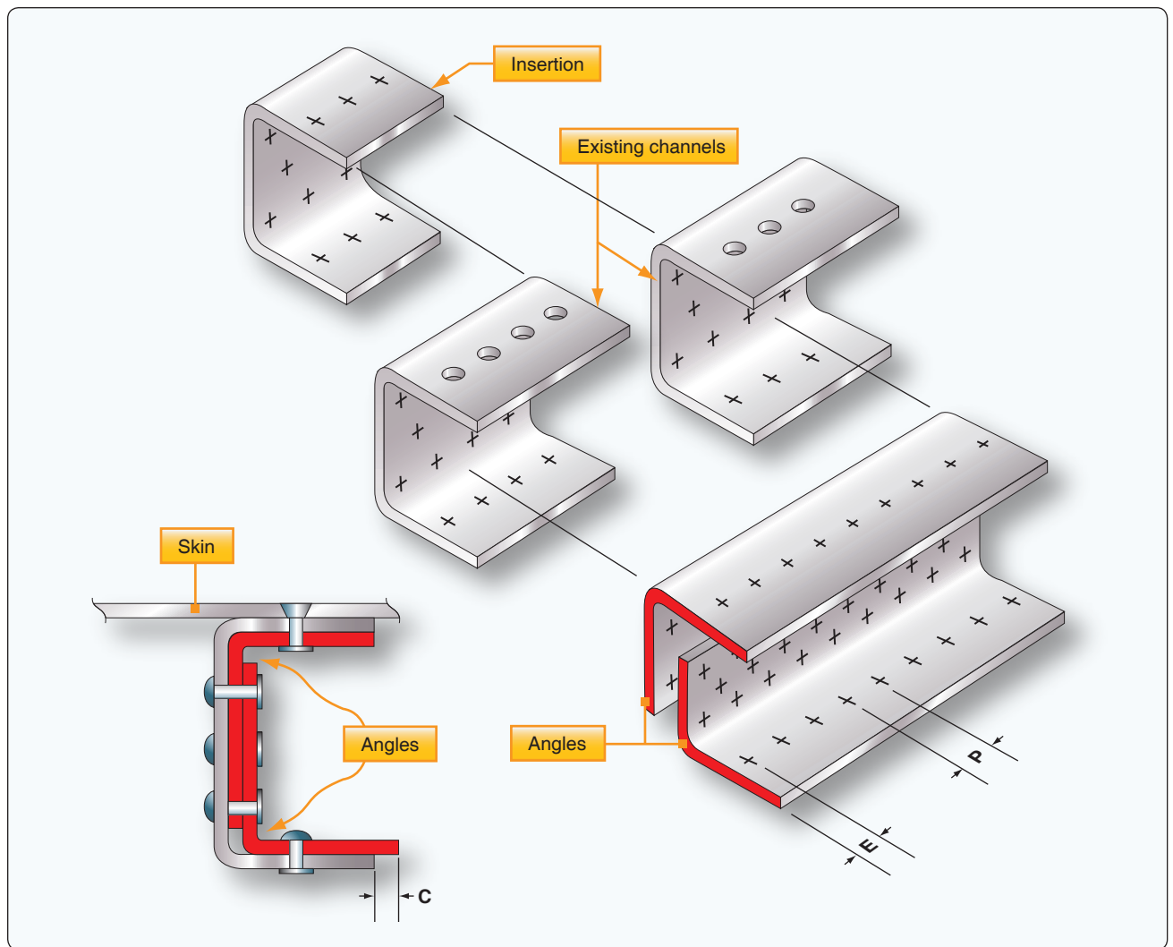
Figure 4-196. U-channel repair.
