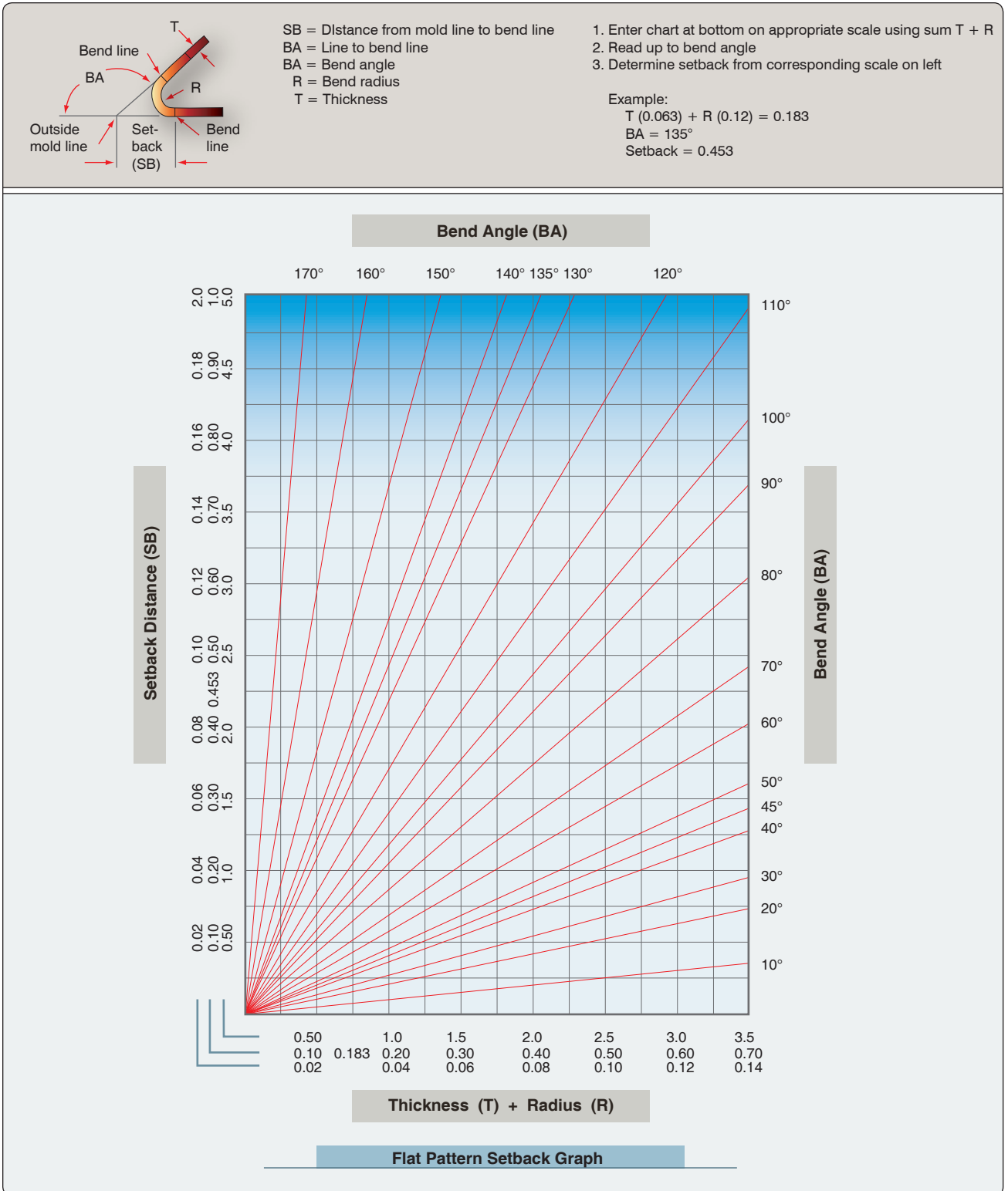
Figure 4-125. Setback chart.
