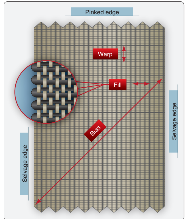
Figure 3-2. Aircraft fabric nomenclature.
