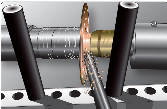
Figure 4-63. Spin forming.
