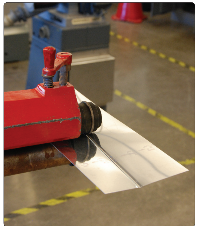
Figure 4-62. Rotary machine.
