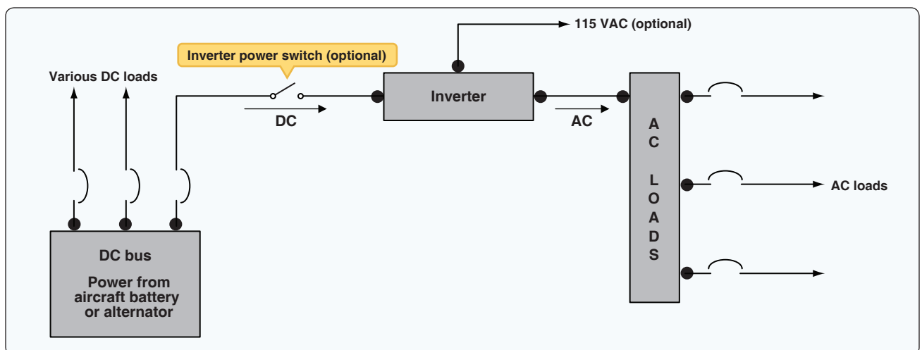
Figure 9-99. Distribution circuit..
