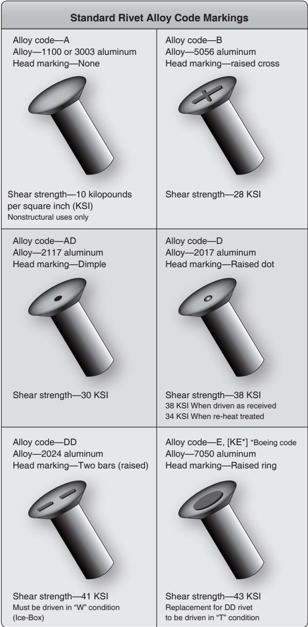
Figure 4-77. Rivet alloy strength.
