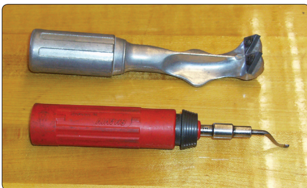
Figure 4-38. Burring tools.
