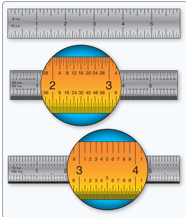
Figure 4-3. Scales.
