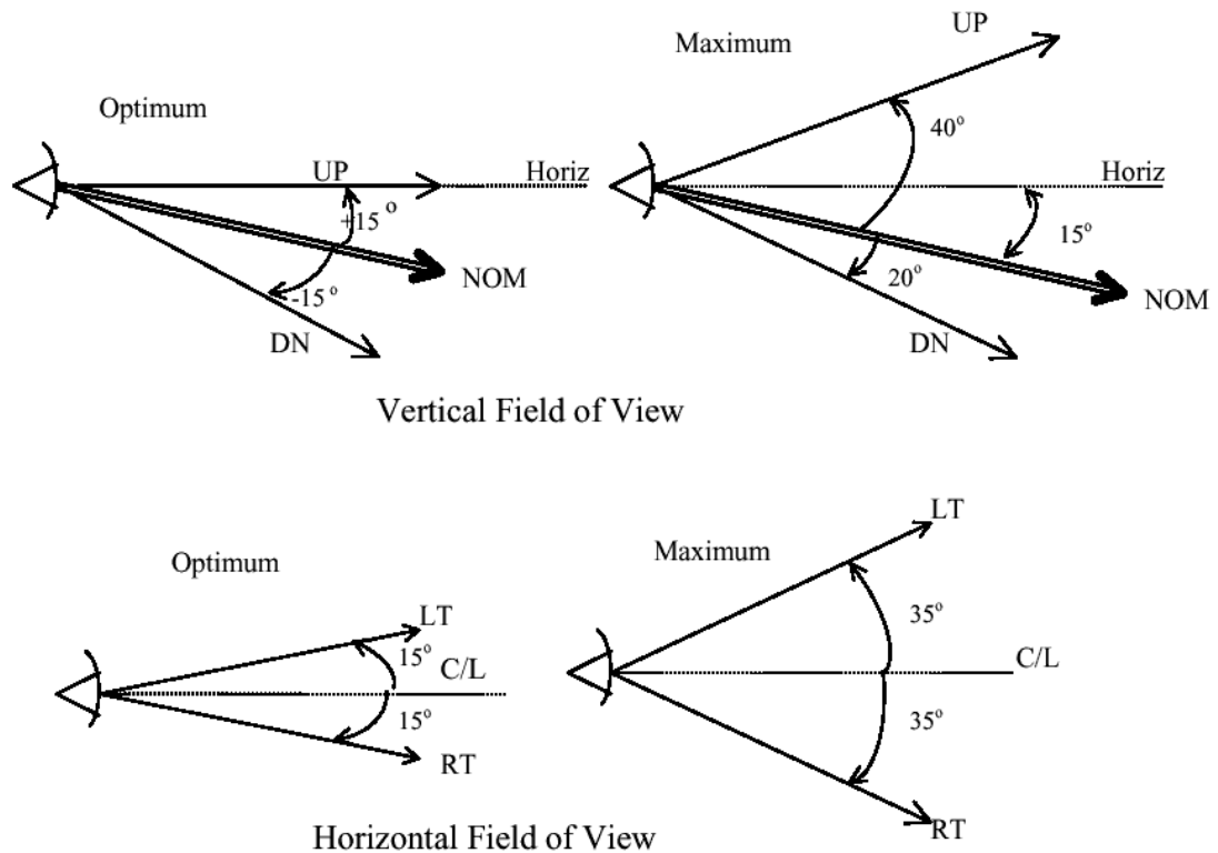
Figure C-2. Primary Field-of-View
